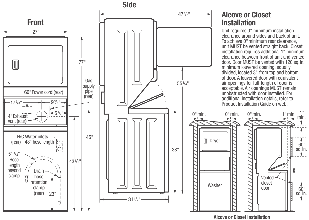
Alcove or Closet Installation
