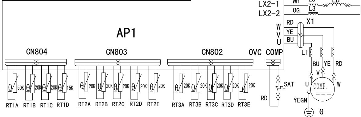
OUTDOOR UNIT
